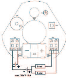
BATTERY POWERED; SWITCH OUTPUT CONNECTED
