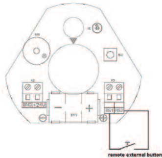
REMOTE SNOOZE WIRING SHOWN BATTERY POWERED CAN BE COMBINED WITH LINE POWER
