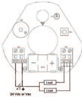
24 VAC/VDC LINE POWER WIRING; SWITCH OUTPUT CONNECTED BATTERY ACTS AS BACK-UP POWER
