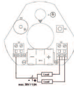
24 VAC/VDC LINE POWER; SWITCH OUTPUT CONNECTED SEPARATE POWER FOR SUPPLY WITH SWITCH LOOP
